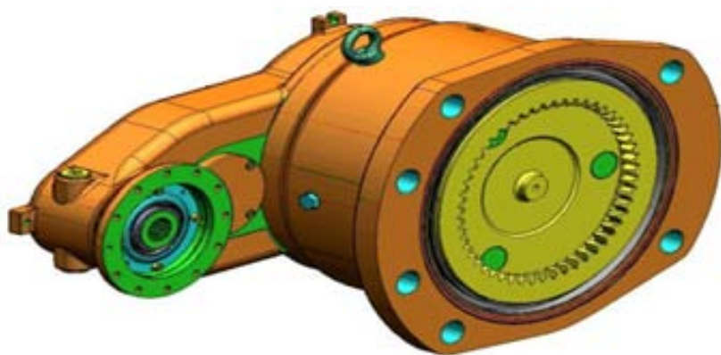
行走齿轮箱/TRACK GEARBOX
