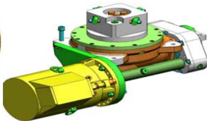
装载齿轮箱/LOADER GEARBOX
