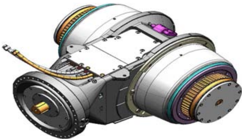
截割齿轮箱/CUTTER GEARBOX
